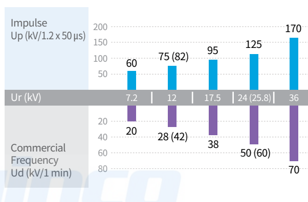
Standard of Withstand Voltage per Rated Voltage Specified in IEC 62271-1
