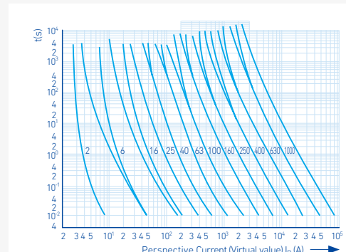
Time-current Range of "gG" Fuse Links
