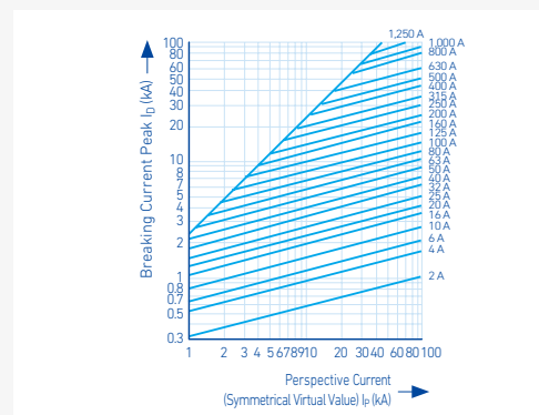
Breaking Current Characteristics Curve of "gG" Fuse Links
