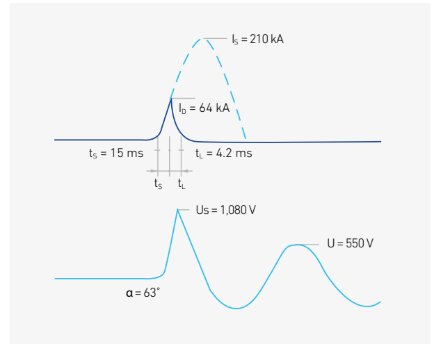
Wave curve of current limiting characteristics of fuse link
