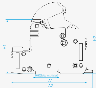
FUSE125
