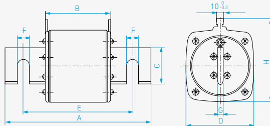
Fuse Link (NT4)
