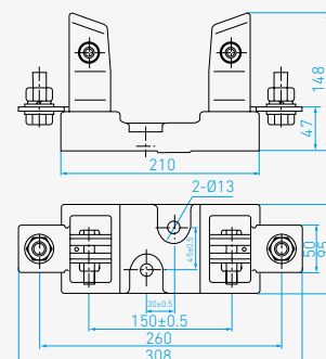
Fuse Base
